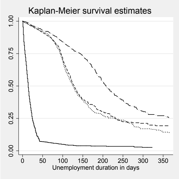
Figure 1: Kaplan-Meier estimates of survival until signing an IA (in dependent right-censoring setting).
