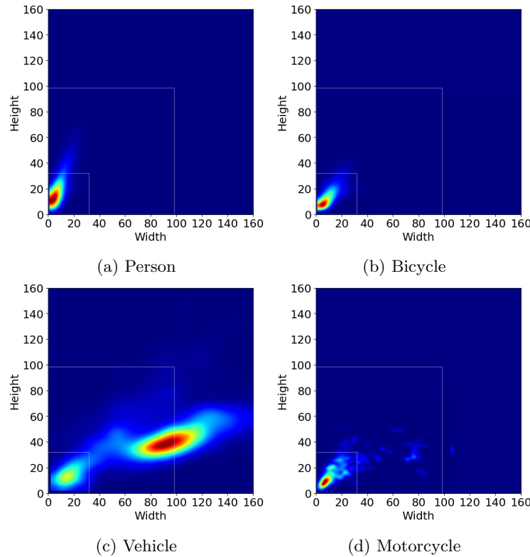
Fig. 3: Illustration of object size (height×width, in pixels) across the dataset. The white outlines separate the areas that would be labeled as small, medium and large following COCO standards.
