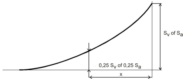
Schets 1
