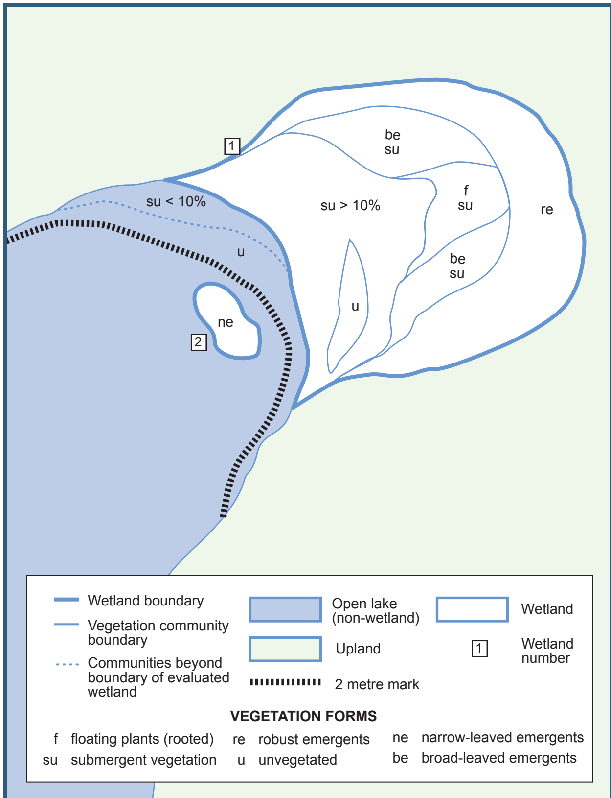
Figure 12: Aerial view showing mapping of vegetation communities and open water boundary of a wetland (see figure 13 for a cross-sectional view).
