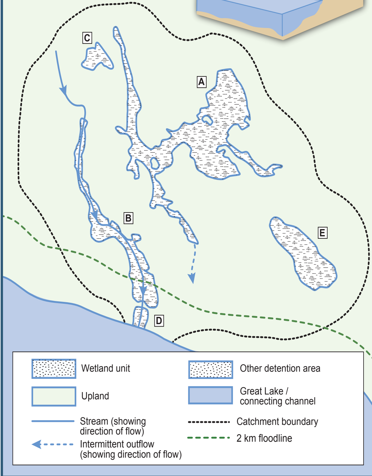
Figure 22: An example of a 4-unit wetland complex for scoring flood attenuation in which both the area of the riverine wetland unit and the lacustrine (at rivermouth) wetland unit are not eligible for scoring under Section 3.1.
