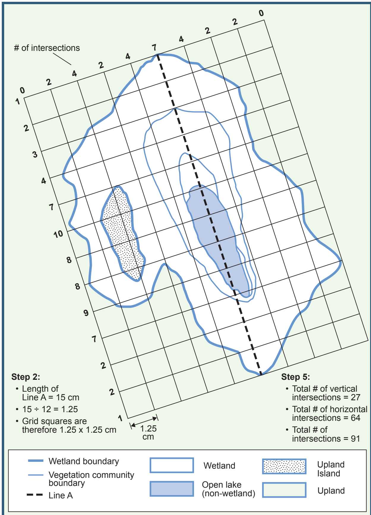
Figure 15: Example of an interspersed grid for a single contiguous wetland.
