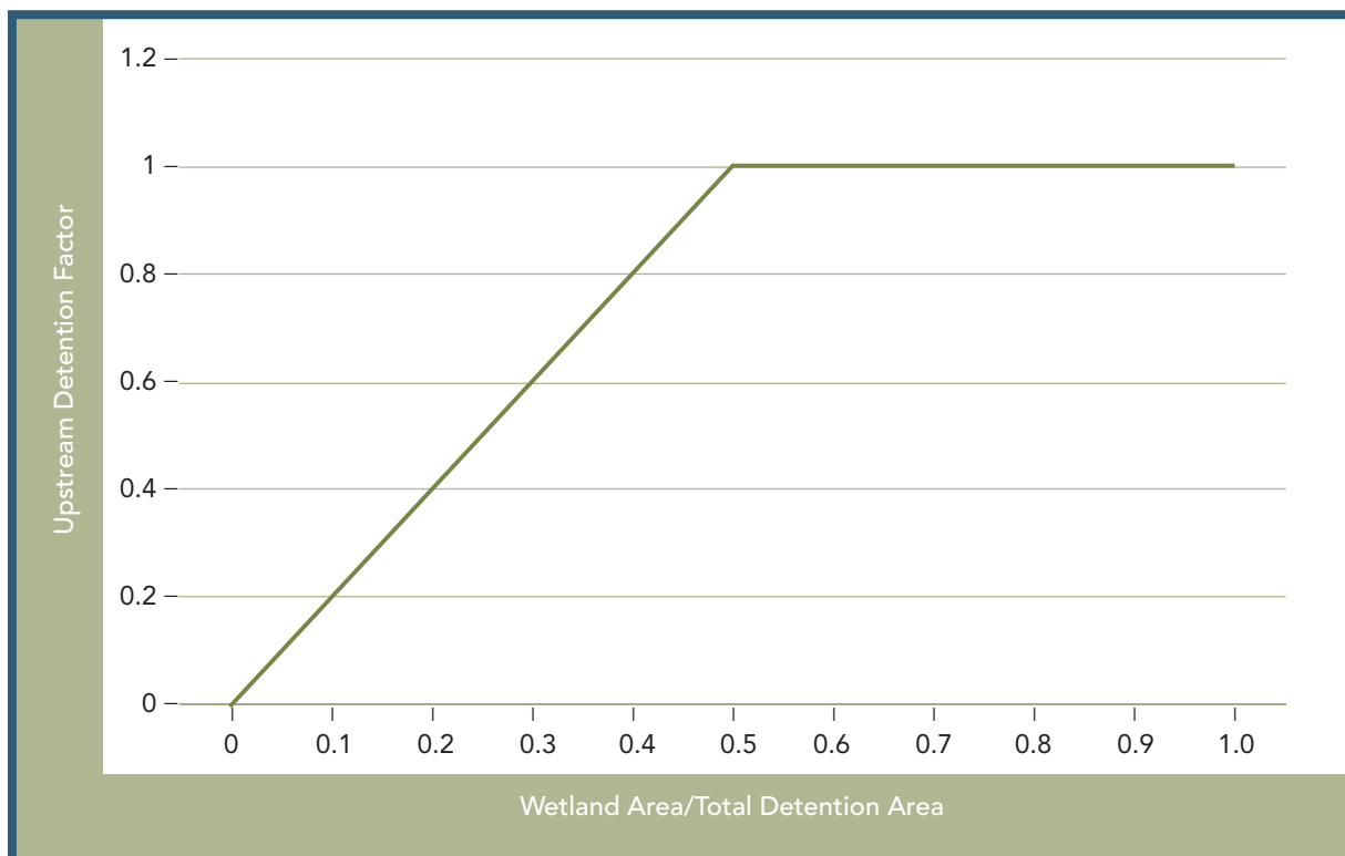
Figure 19: Relationship between upstream detention, wetland area and total detention area.
