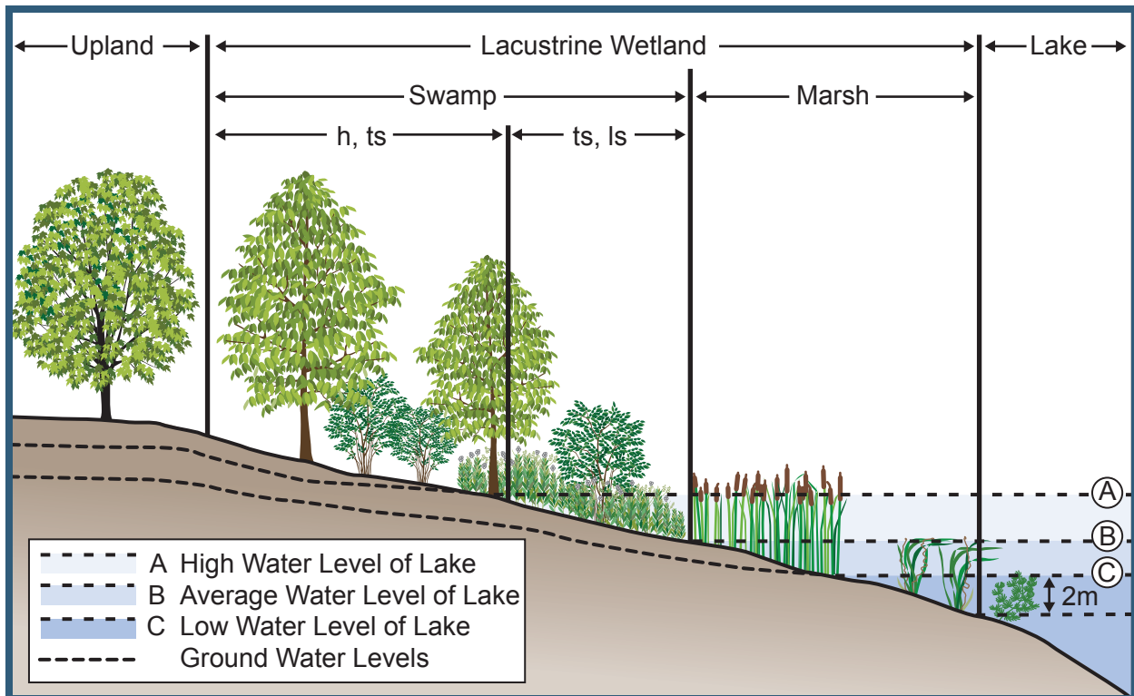
Figure 7: Lacustrine Site Type
