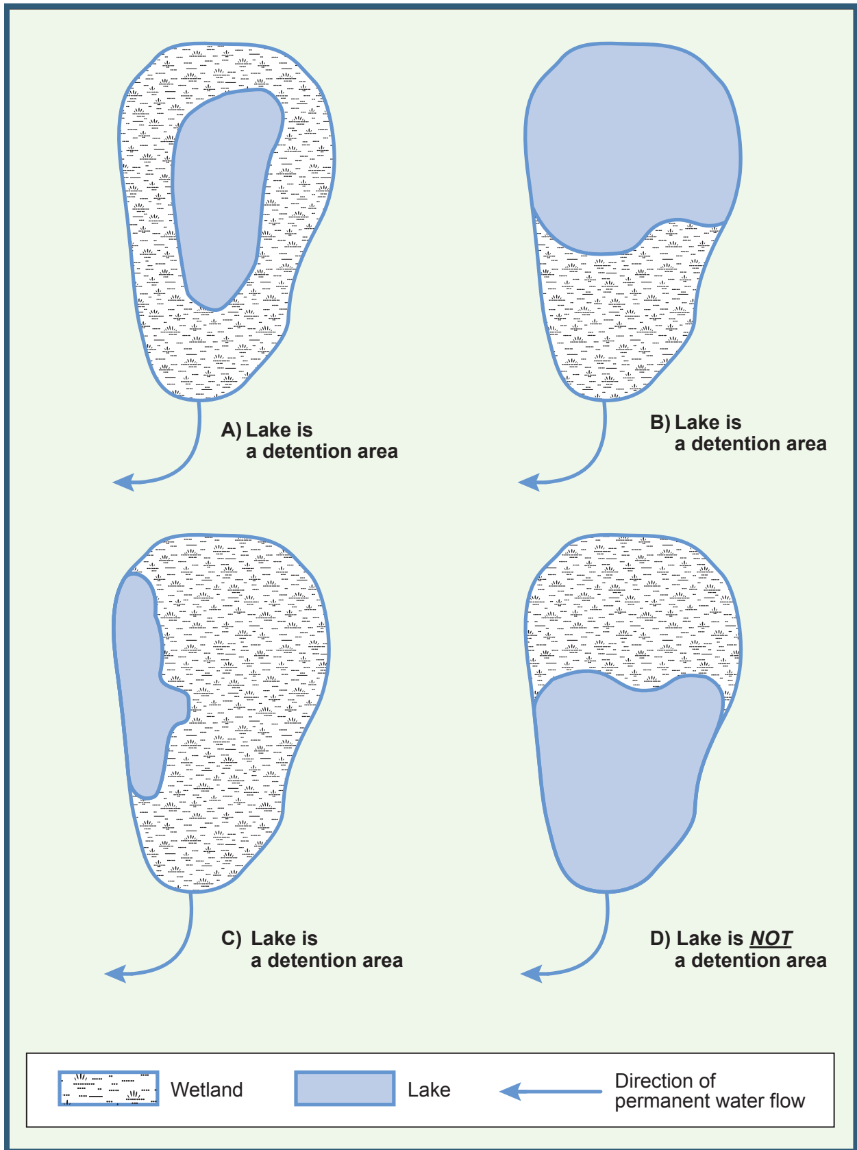
Figure 20: Determination of detention areas – lacustrine wetlands.
