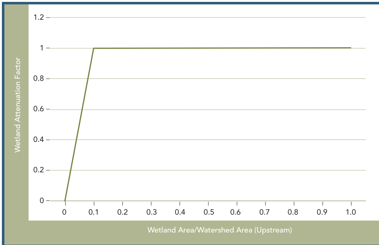
Figure 21. Relationship between wetland area, upstream watershed area and the ability of the wetland to attenuate flood peaks (wetland attenuation factor).
