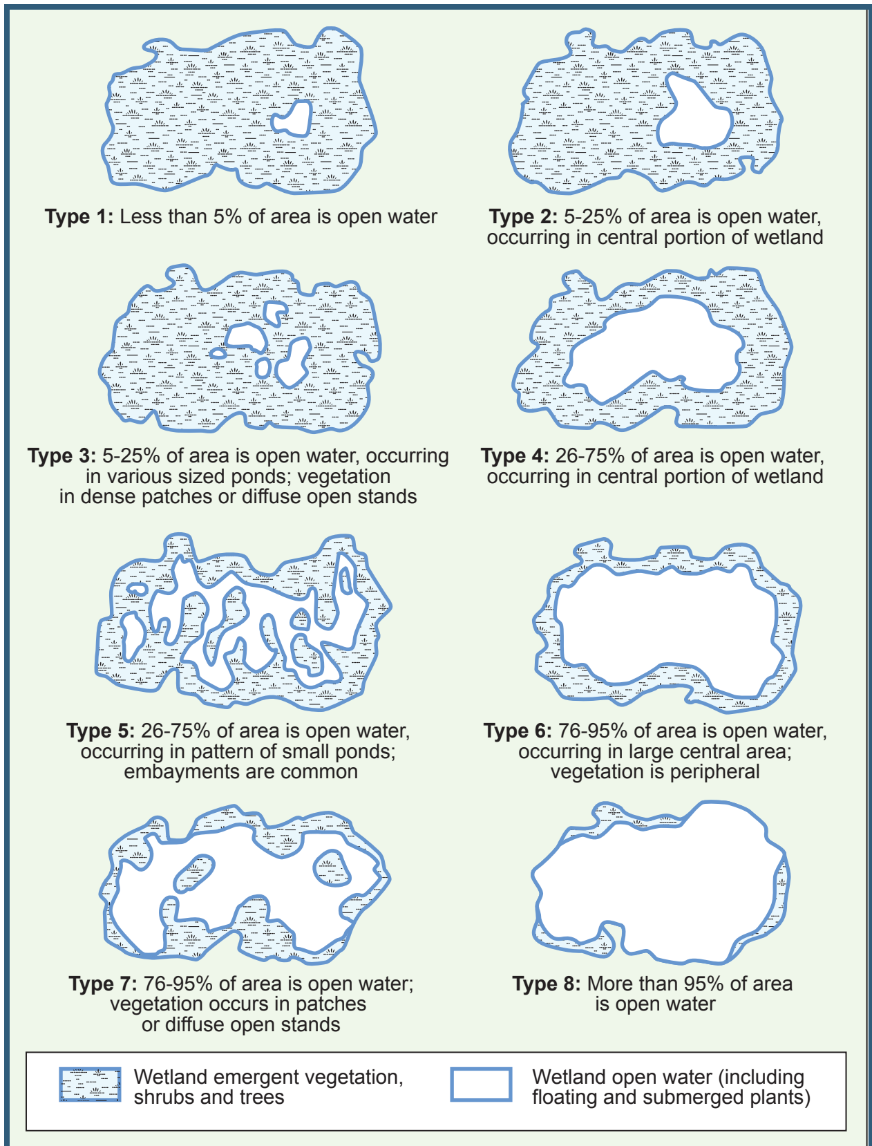
Figure 17: Wetland open water types described in Section 1.2.6.
