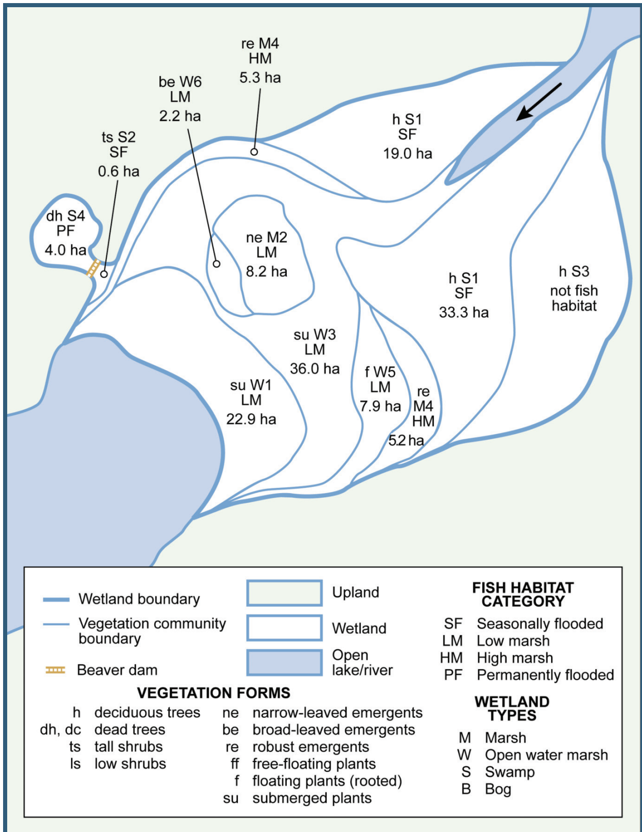
Figure 25: Example of a wetland being assessed for spawning and nursery habitat
