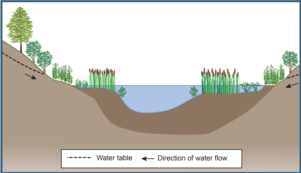
Figure 23b: Groundwater discharge. Water inflow from surrounding lands into a wetland occurs when the water level of a wetland is lower than the surrounding water table. Wetlands often act as discharge areas in the spring. Modified from Mitsch and Gosselink (2000).
