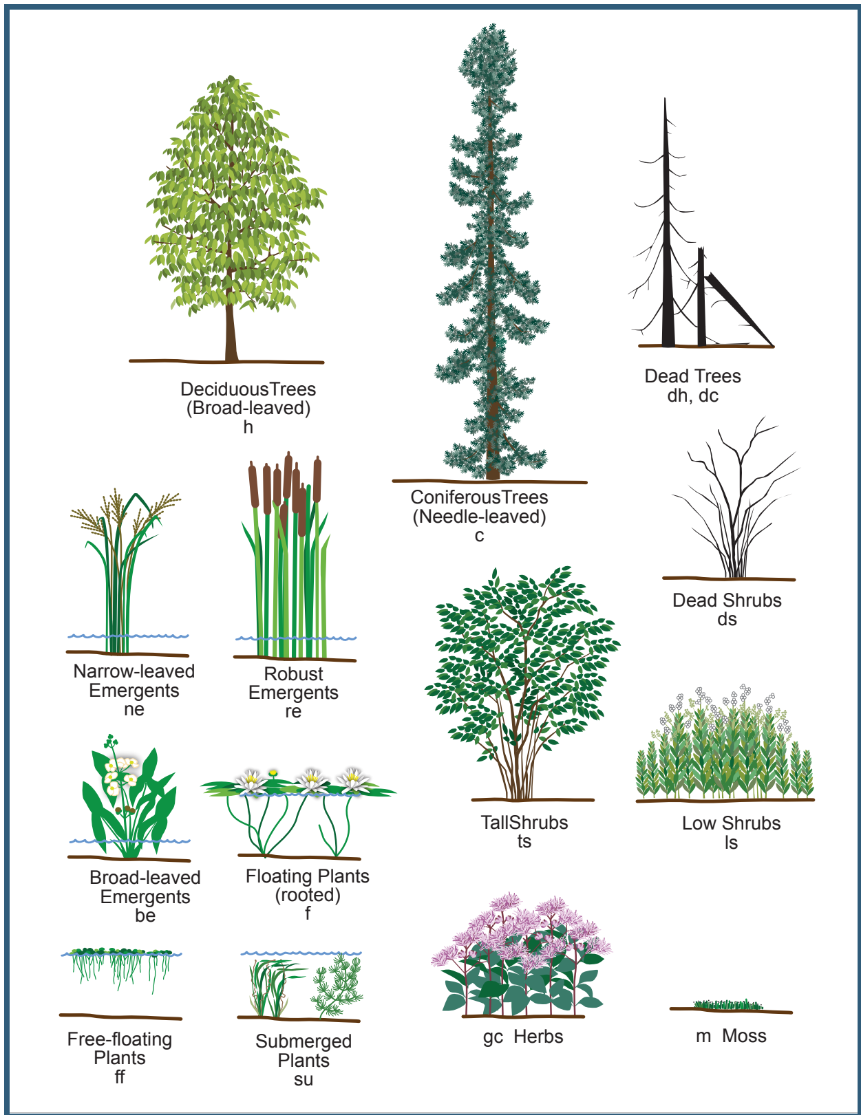
Figure 11: Wetland Vegetation Forms and Symbols
