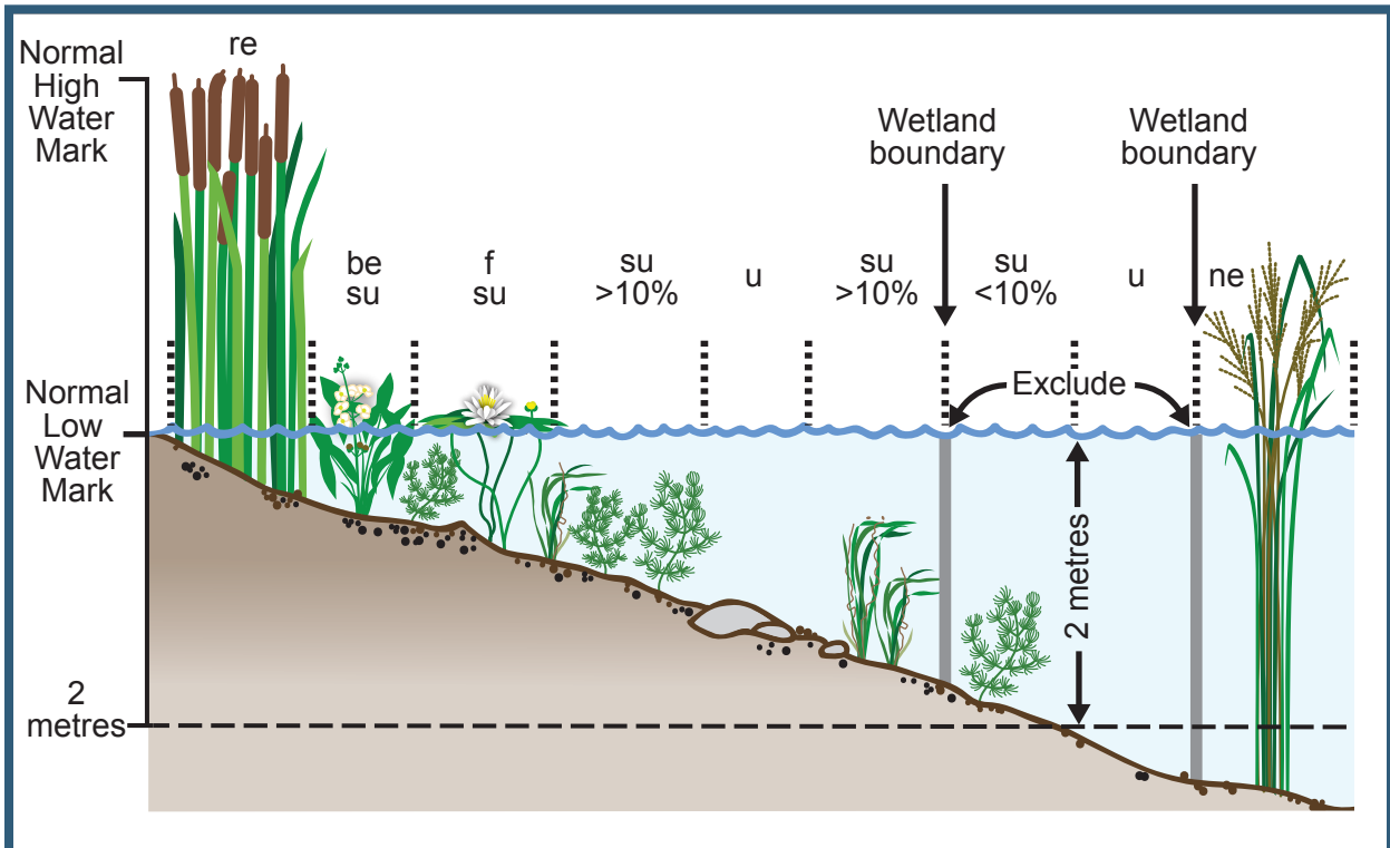
Figure 13: Cross-sectional view of vegetation communities and open water boundary of a wetland (see figure 12 for an aerial view).
