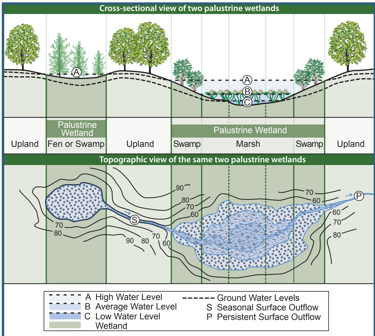
Figure 9: Palustrine Site Type
