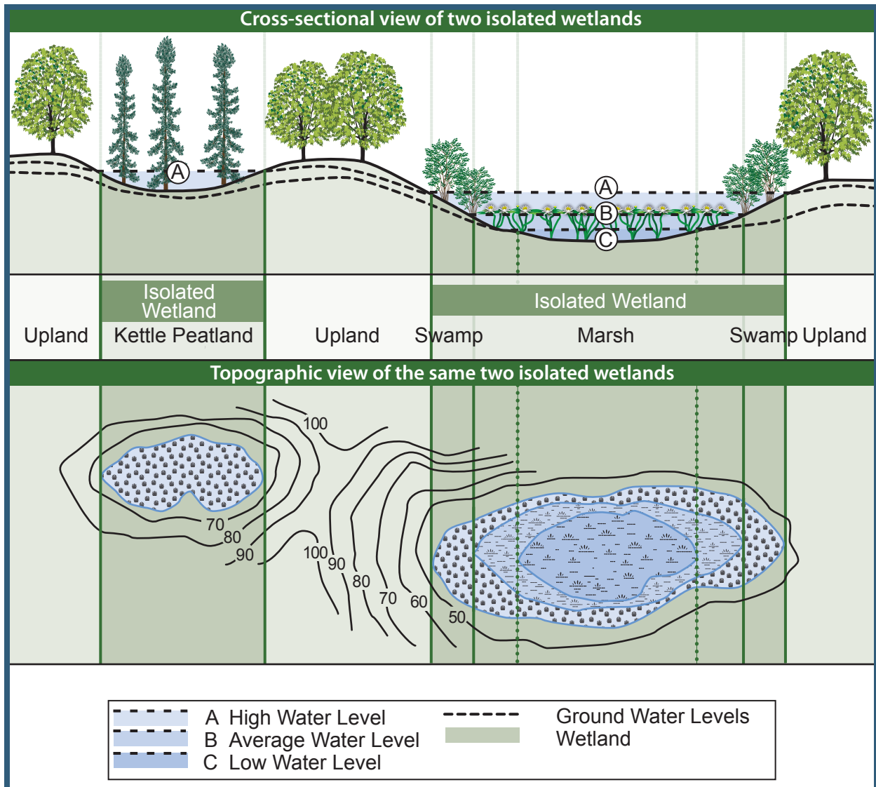
Figure 10: Isolated Site Type
