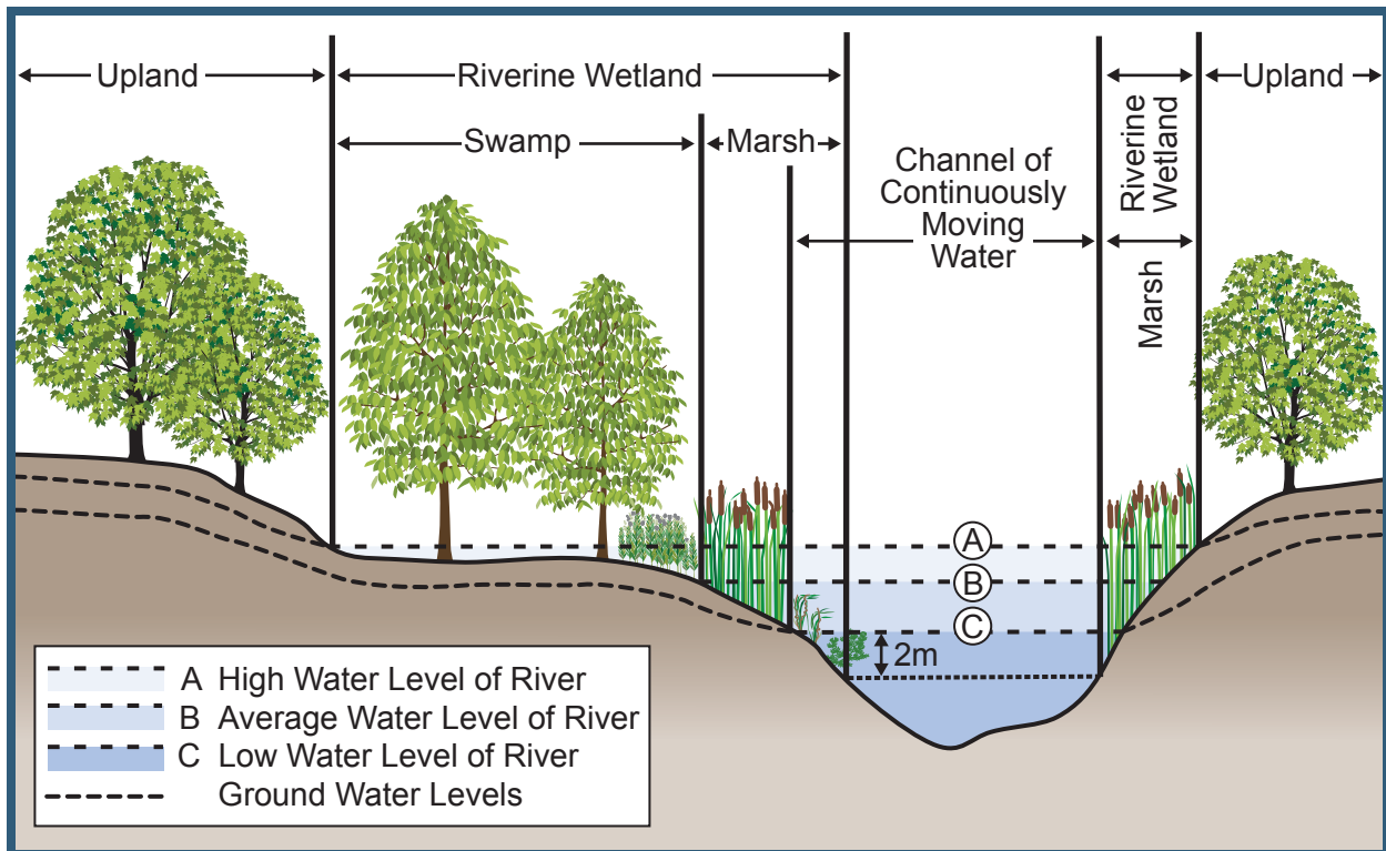
Figure 8: Riverine Site Type
