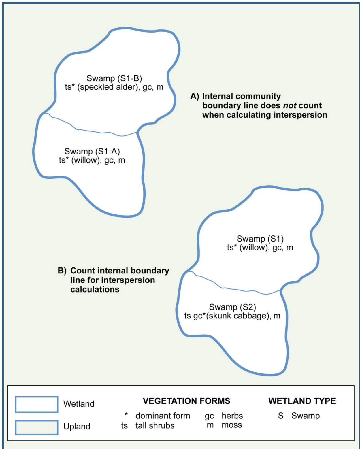
Figure 14: Example of how to use internal vegetation boundaries to score diversity of forms and interspersion. A) The two swamp communities illustrated are dominated by ts and are considered the same for purposes of scoring diversity of forms and interspersion. B) The two swamp communities, one dominated by ts and one dominated by gc, are considered separate communities when scoring diversity of forms and interspersion. Refer to Sections 1.2.2 and 1.2.5 in text for details.
