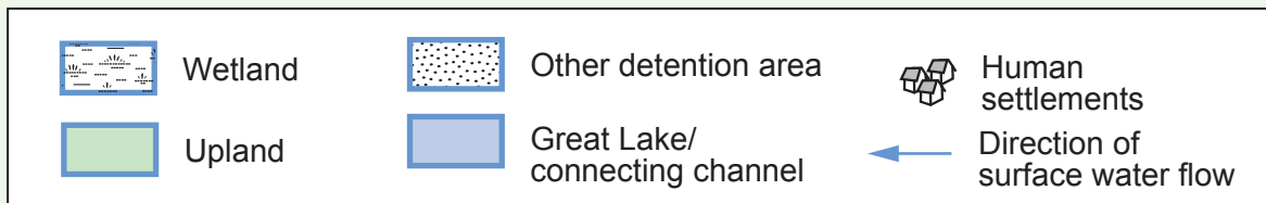
Figure 18: Wetlands with and without flood attenuation value under the OWES.
